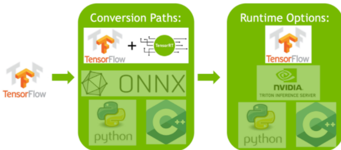
Figure 6. TF-TRT integration with TensorRT.
