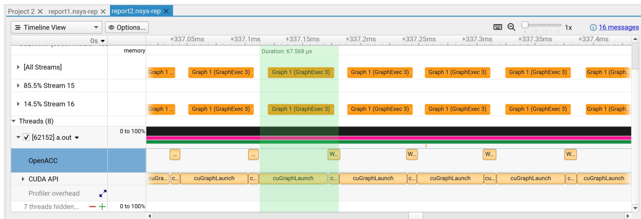
Figure 2: Nsight Systems Report2 Timeline
