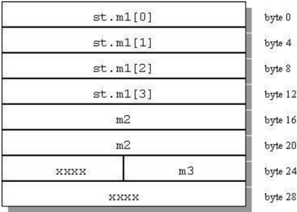
Figure 2 Tail Padding in a Structure
