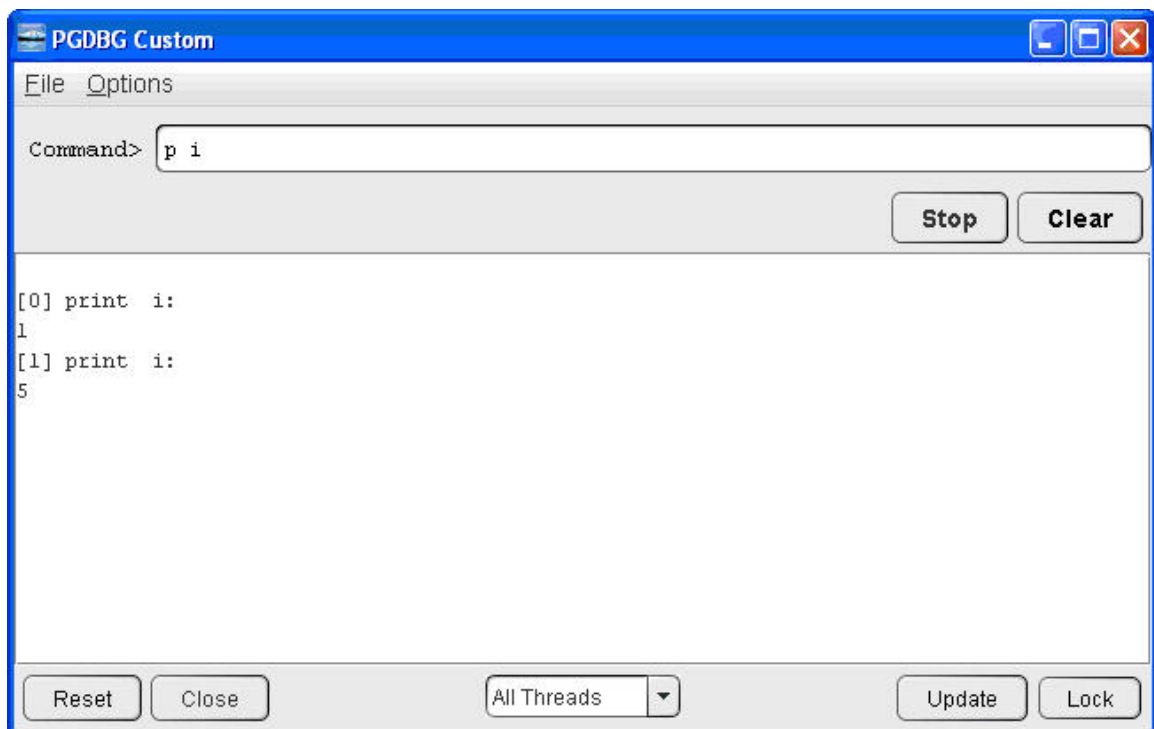
Figure 22 OpenMP Private Data in Debugger GUI
