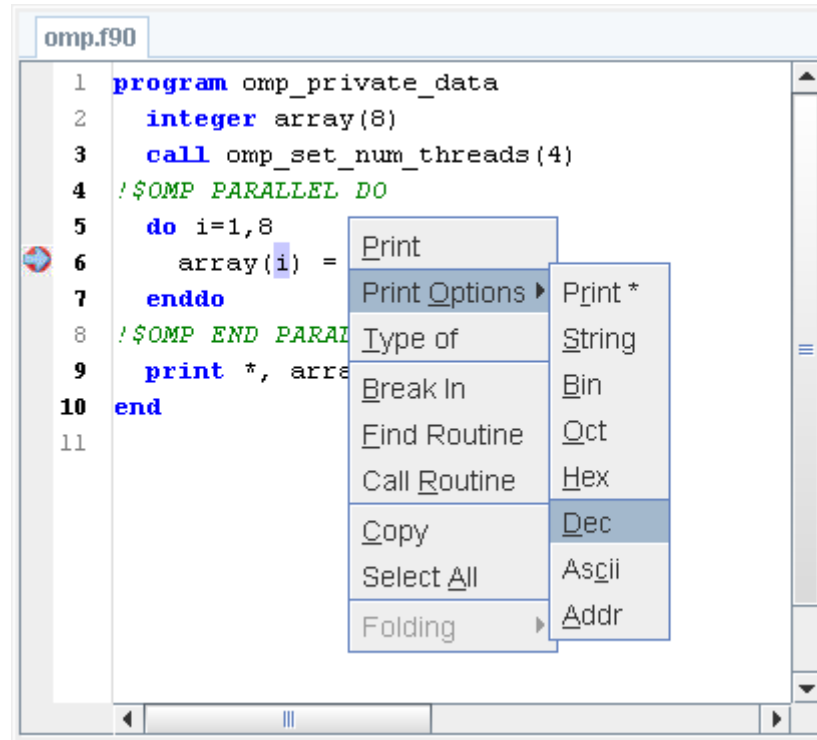
Figure 3 Context Menu
