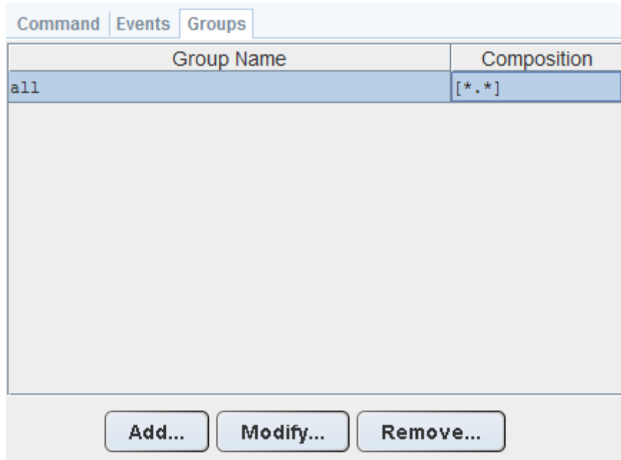
Figure 20 Groups Tab
