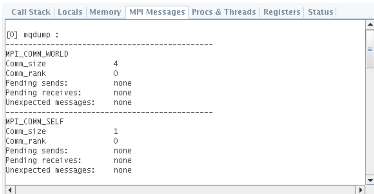
Figure 2.15. MPI Messages Tab
