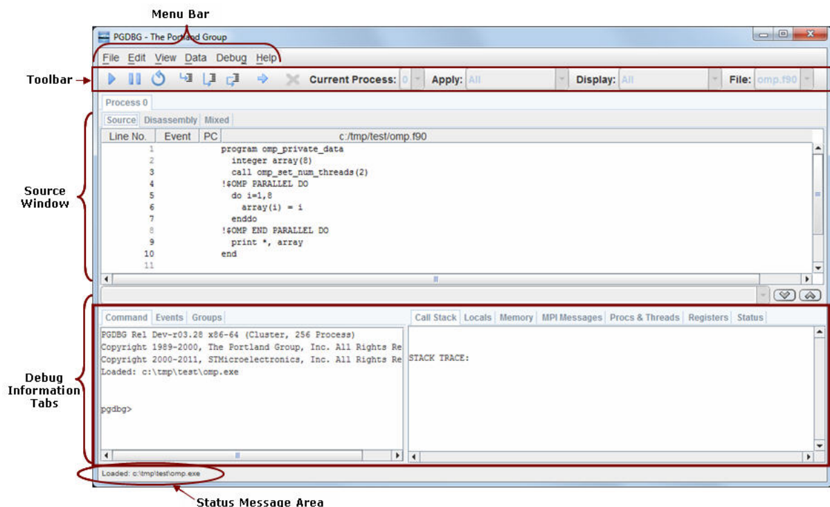
Figure 2.1, “Default Appearance of PGDBG GUI” shows the PGDBG GUI as it appears when PGDBG is invoked for the first time.
