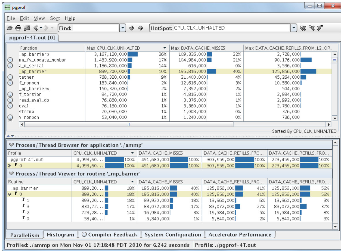
Figure 2.11. Profile with Hardware Event Counter
