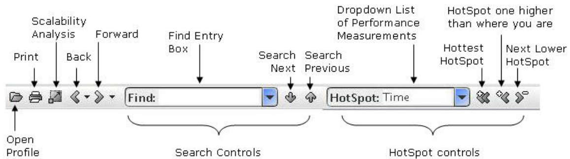
Figure 7.2. PGPROF Toolbar
