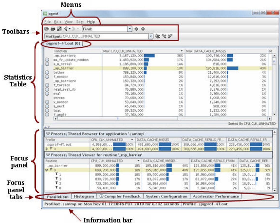
Figure 2.1. PGPROF Overview
