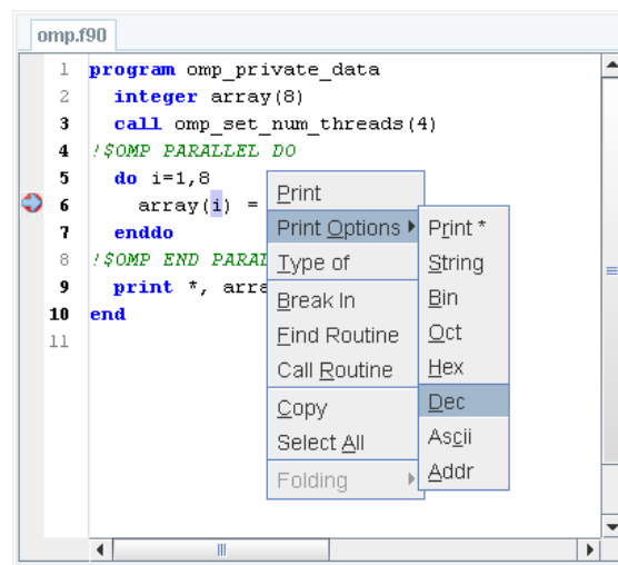
Figure 2.3. Context Menu
