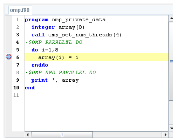
Figure 2.2. Source Window
