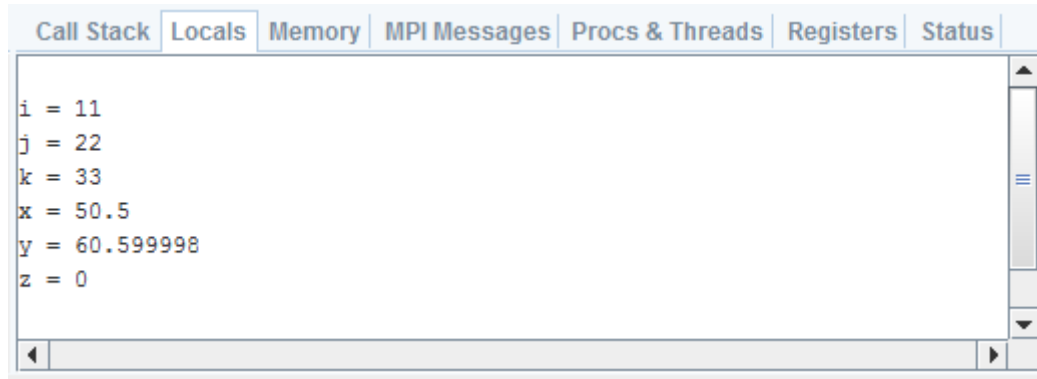
Figure 15 Locals Tab
