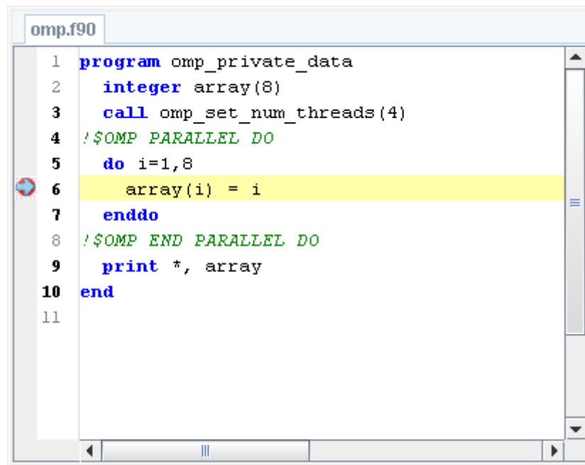
Figure 4 Source Window
