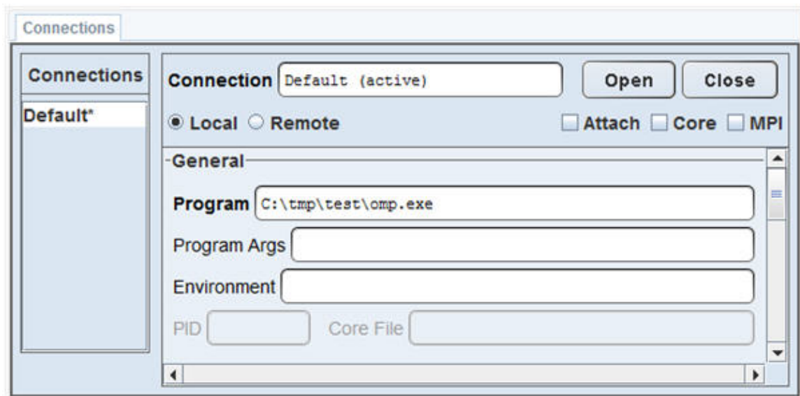
Figure 12 Connections Tab
