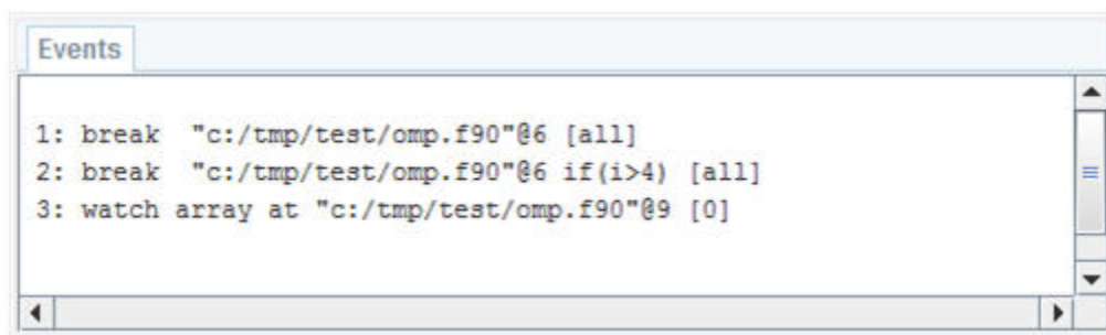
Figure 10 Events Tab
