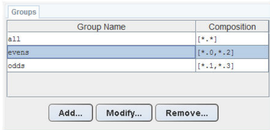
Figure 11 Groups Tab
