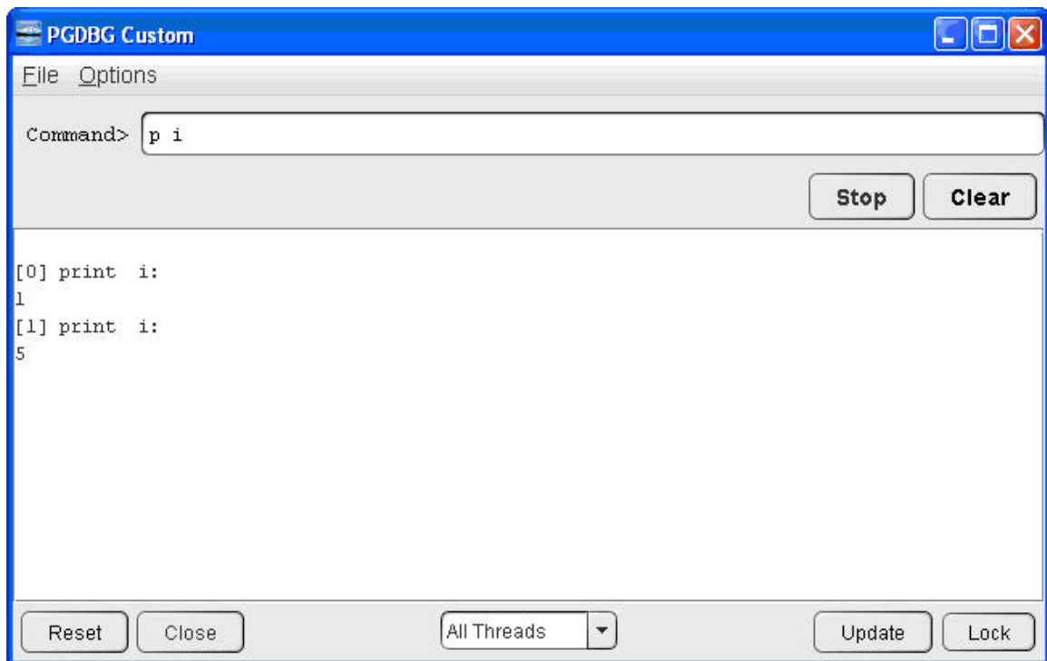
Figure 22 OpenMP Private Data in PGDBG GUI
