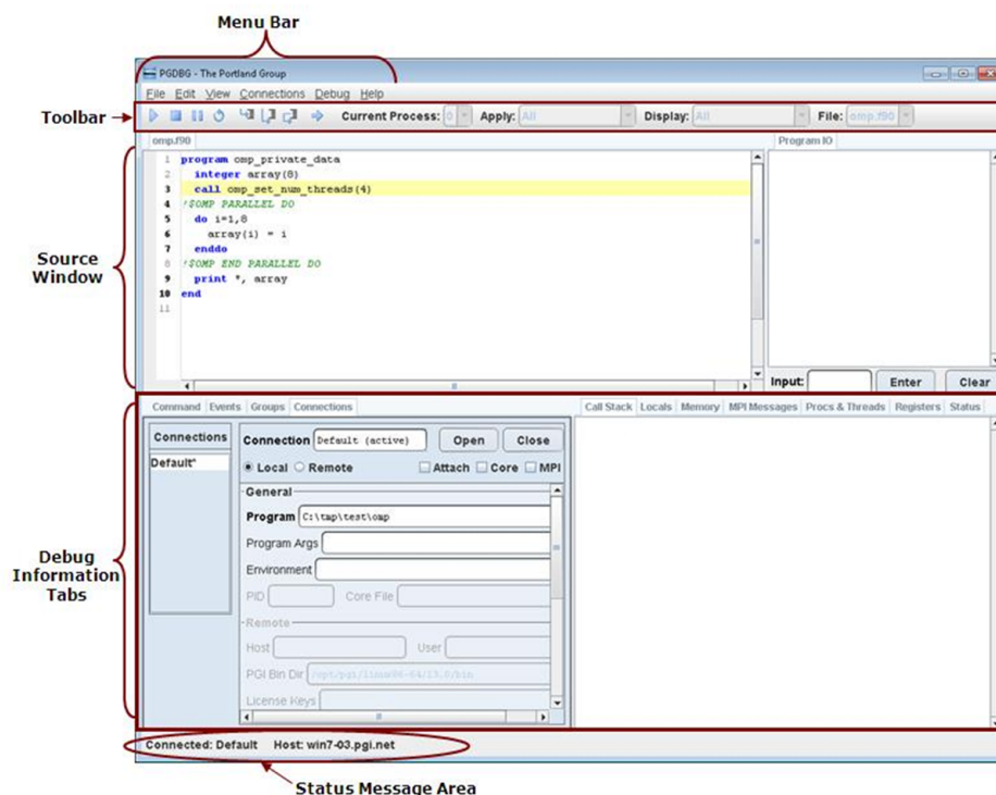
Figure 1 Default Appearance of PGDBG GUI
