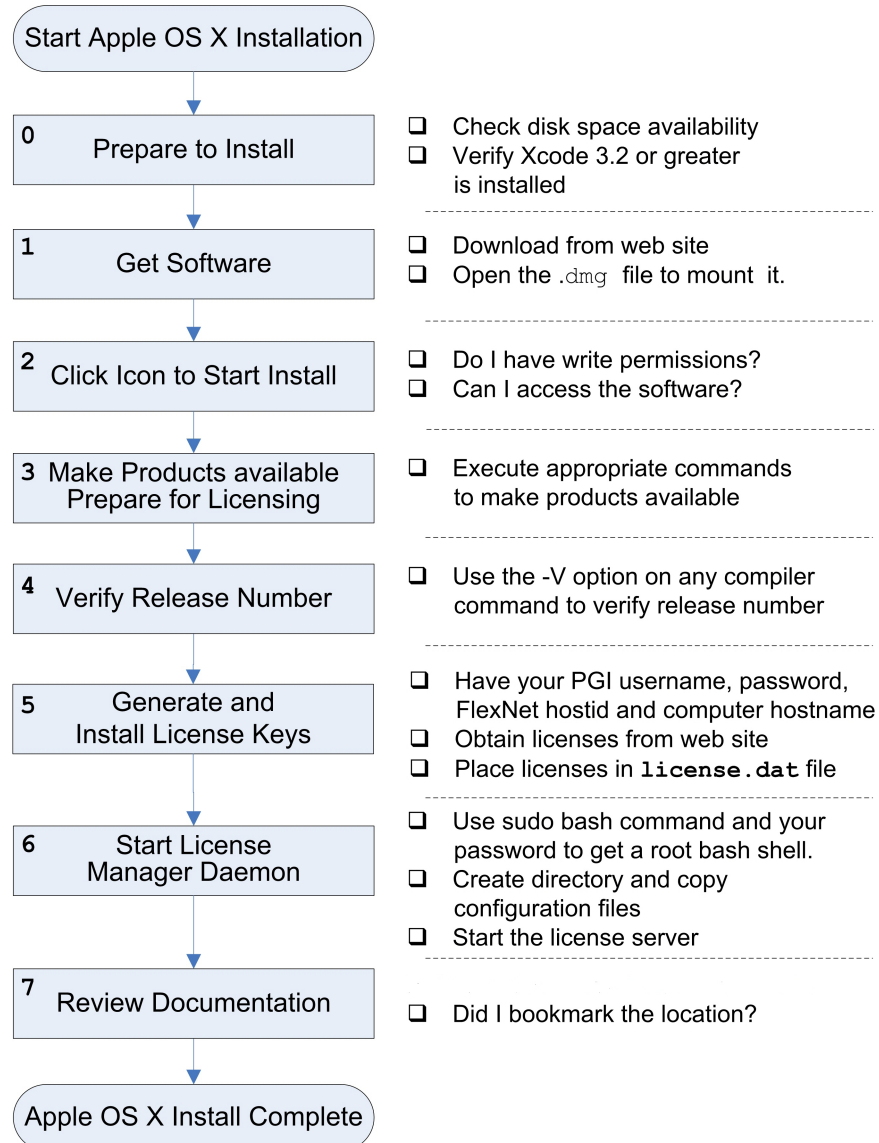
Figure 3 Apple macOS Installation Overview
