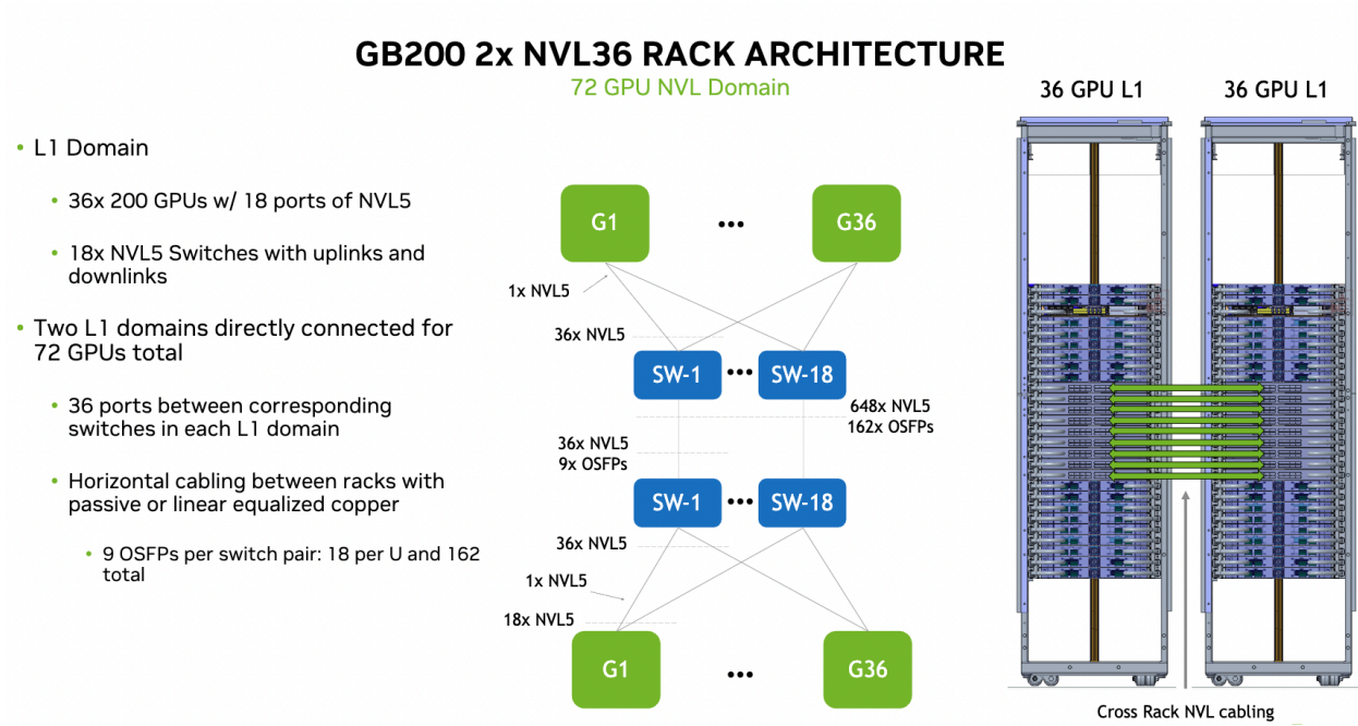
Figure 2 shows the GB200 NVL72 platform with 18 compute trays and nine switch trays.
