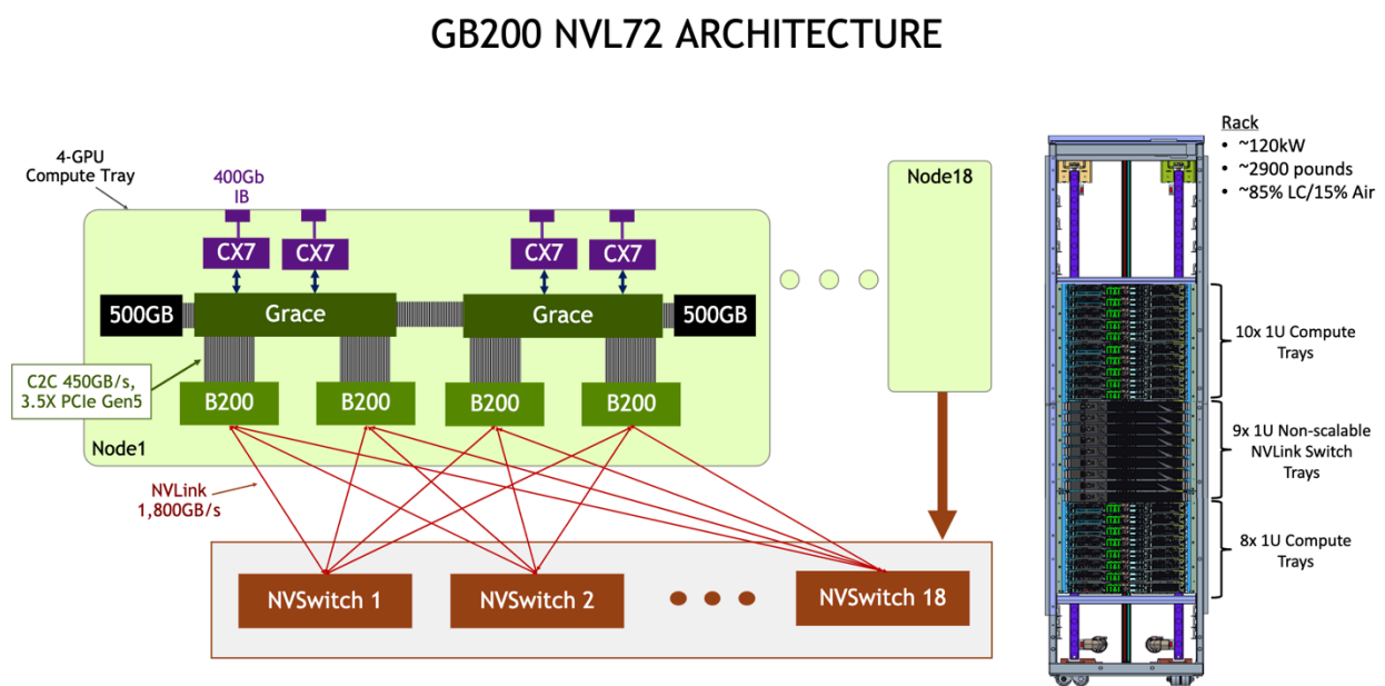
Figure 2. The GB200 NVL72 Platform with 18 Compute Trays and Nine Switch Trays
