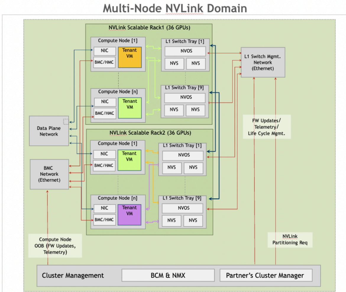
Figure 4. Multi-Node NVLink Domain
