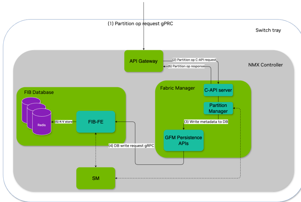
Figure 5. Partition Metadata
